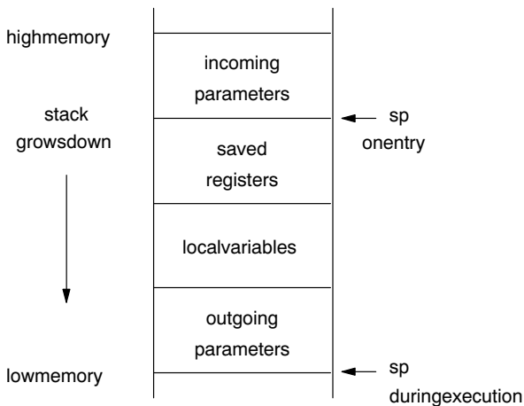
Figure 4-1: Stack diagram
