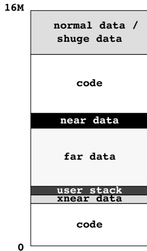
Figure 3-5: Huge memory map example
