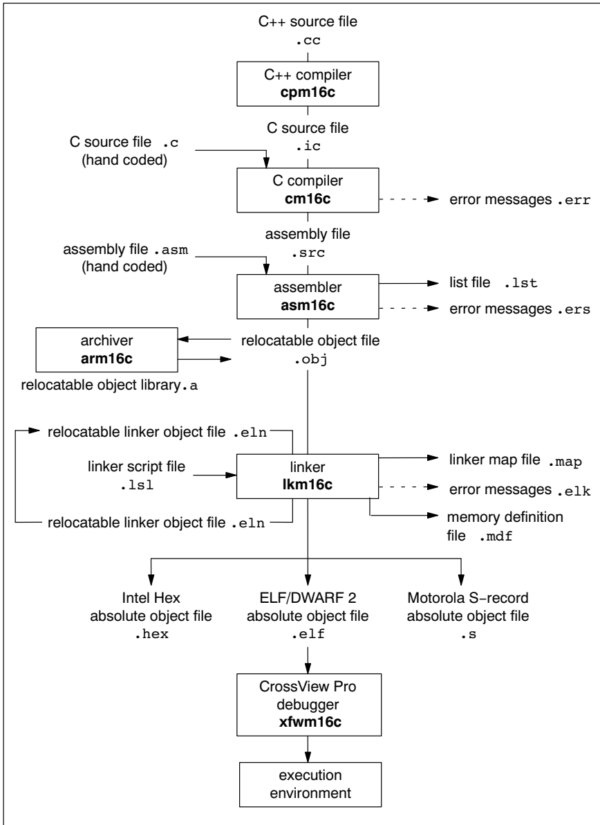
Figure 1-3: Toolchain development flow
