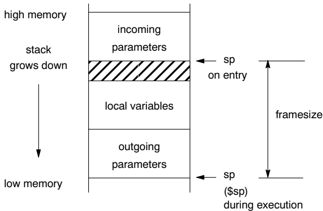
Figure 6-1: Stack frame layout
